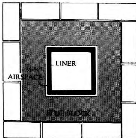
MASONRY CHIMNEYS
