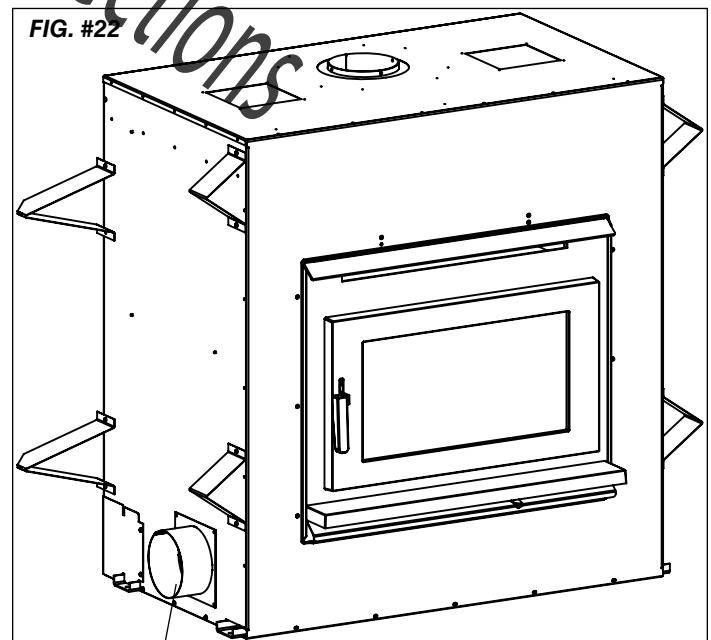
GRAVITY HEAT DUCT AIR INLET. used only when two gravity vents and/or your facing material is more than 3/4"(19mm) thick(Max. 4"(102mm)), NOT RELATED TO CHASE AIR INLET
